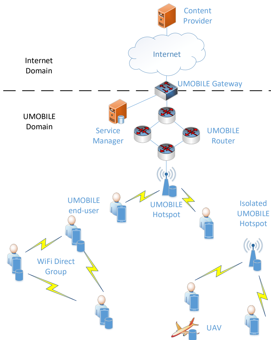
FIGURE 7 – POTENTIAL DEPLOYMENT SCENARIO OF THE UMOBILE PLATFORM
