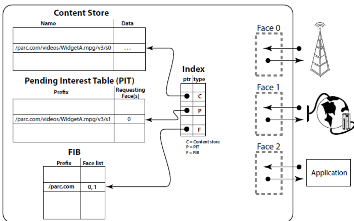
FIGURE 1 - NDN ARCHITECTURE [18]
