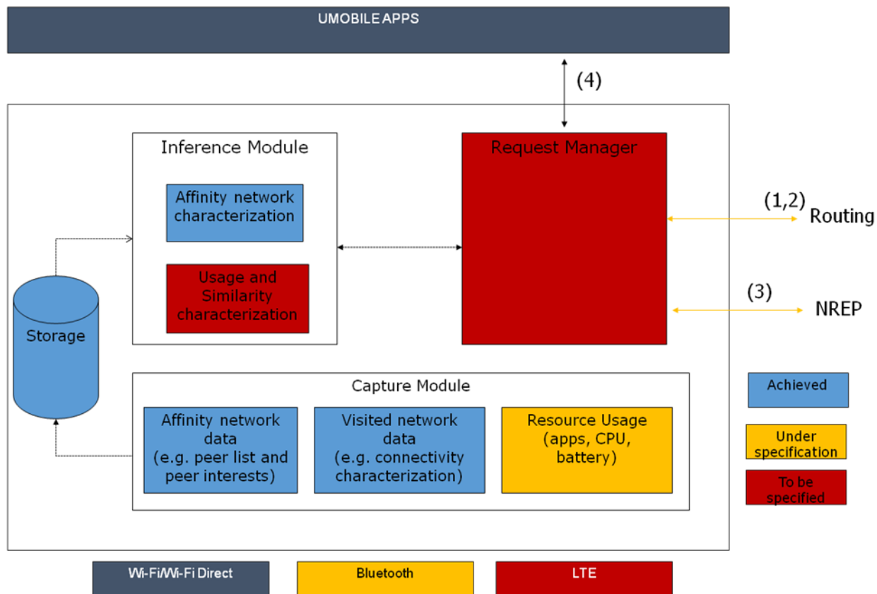
FIGURE 16 - UMOBILE CONTEXTUAL INFORMATION MODULE
