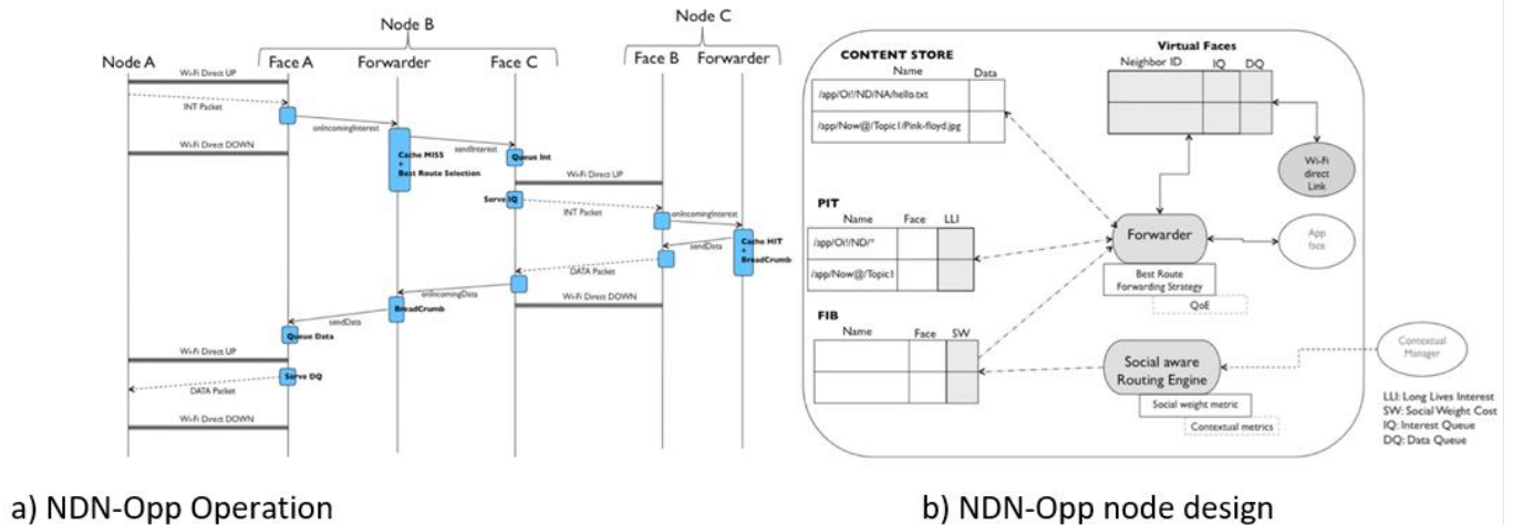
FIGURE 15- NDN-OPP ILLUSTRATION
